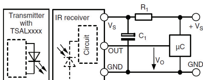
Figure 21: Block diagram of an infrared remote control system. (Source: Mouser Electronics, 2013)
