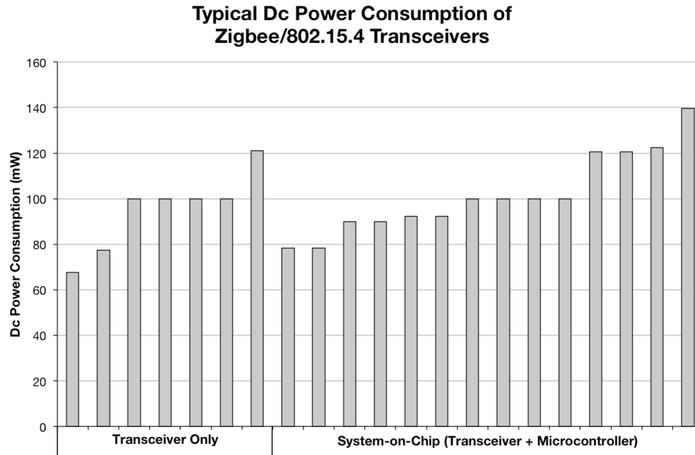
Figure 12: Transmit/receive power consumption for current Zigbee transceiver and SoC solutions
