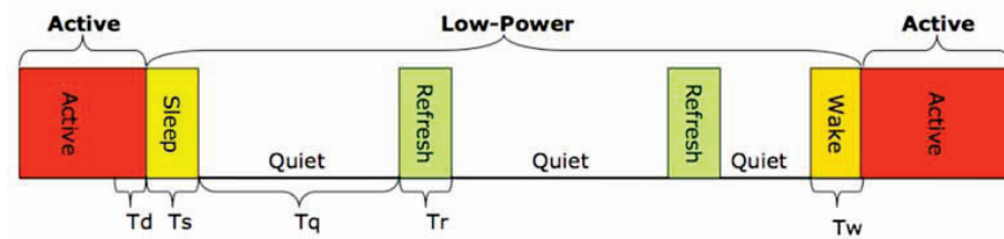
Figure 4: EEE sleep scheduling. (Source: Lawrence Berkeley National Laboratory)
