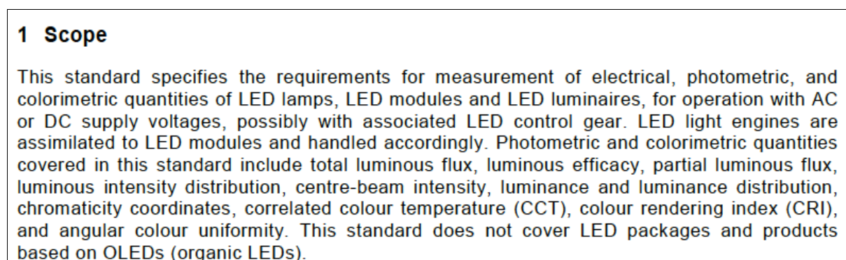
Figure 1. Scope of Coverage of CIE S 025/E:2015
